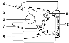
Media path
